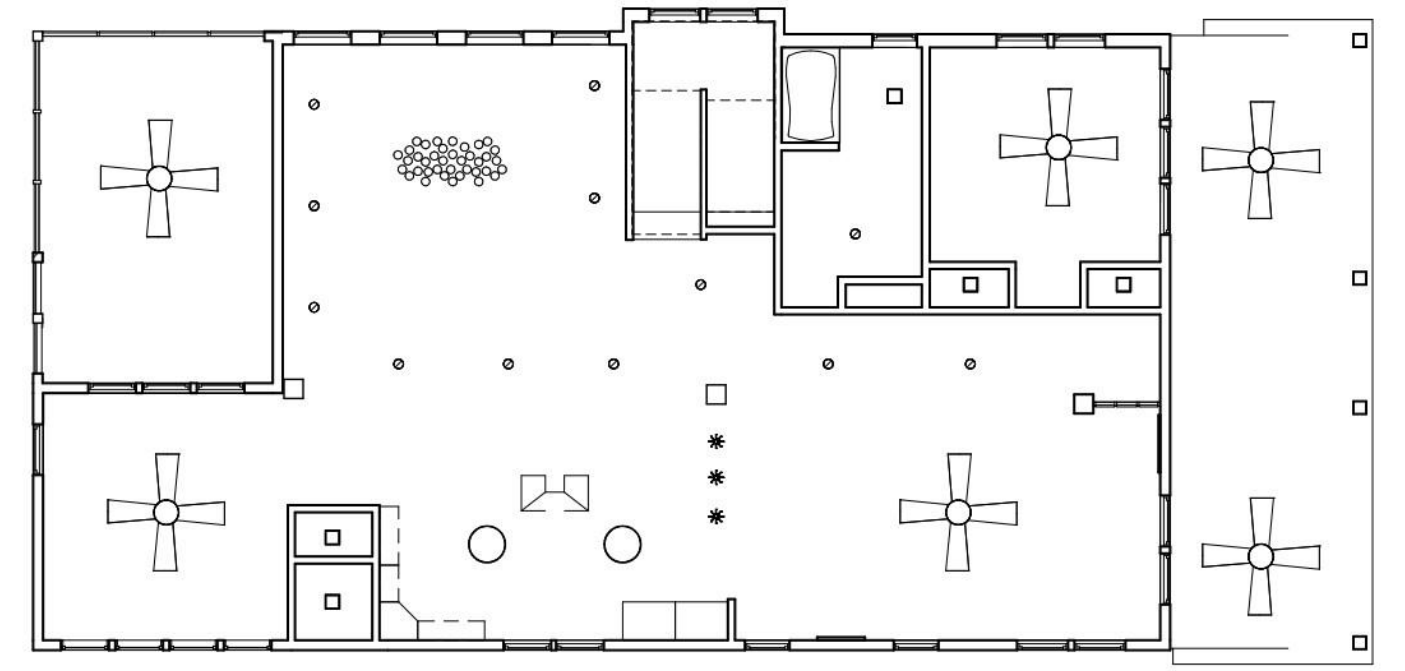
Reflective Ceiling Plan
