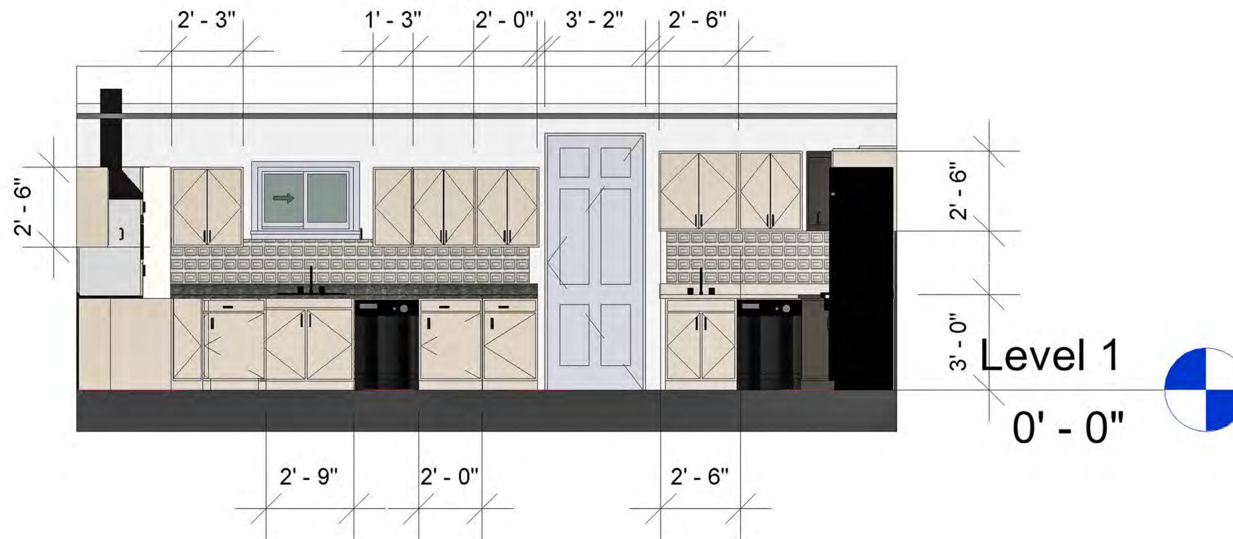
ELEVATION/RENDERING OF KITCHEN
