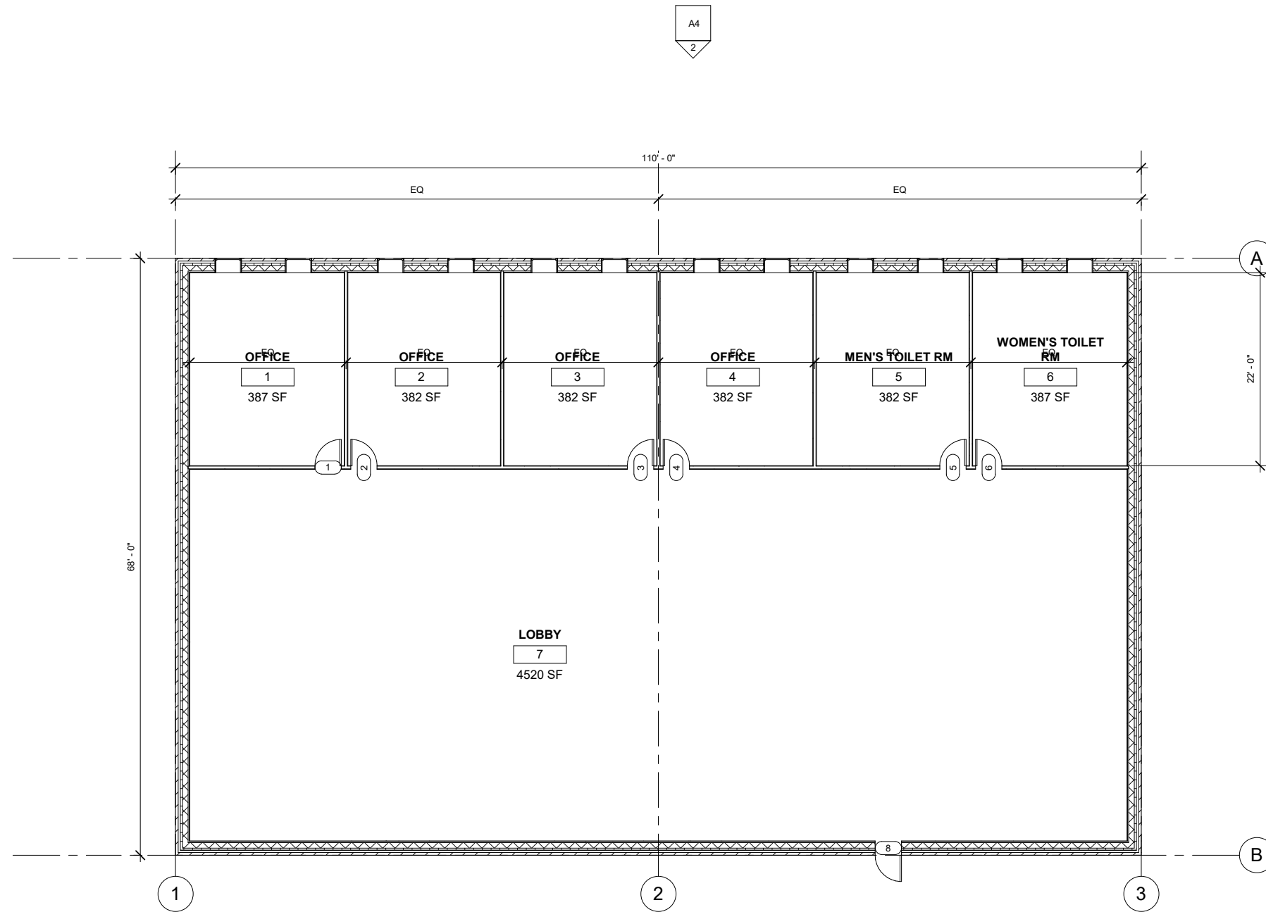
OFFICE BUILDING - OPTION A
