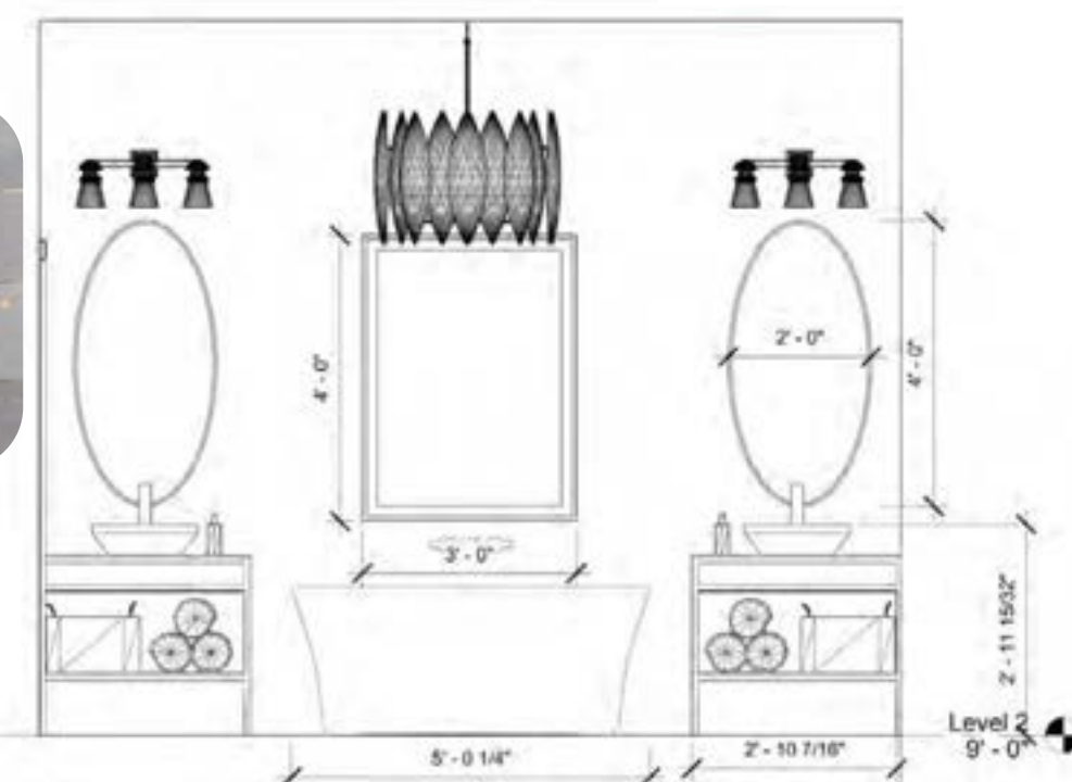
Upstairs Bathroom Elevation - Vanity + Bathtub
