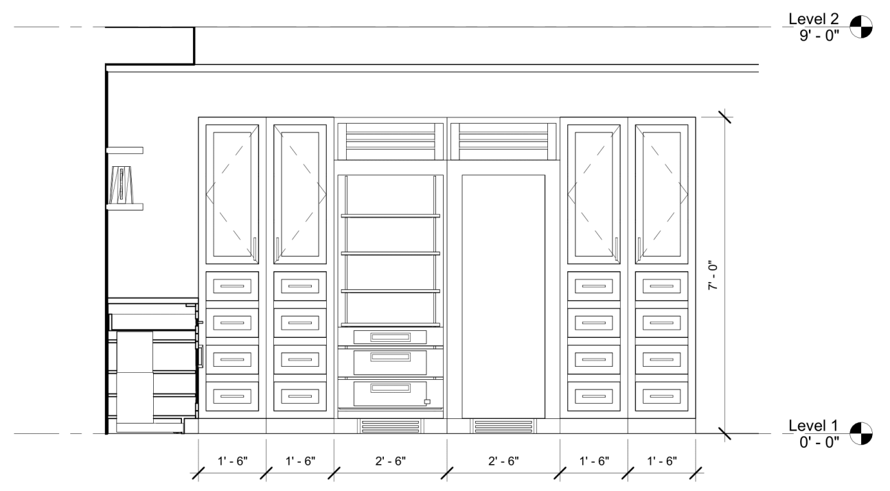
Kitchen Elevation - Short Side of Kitchen
