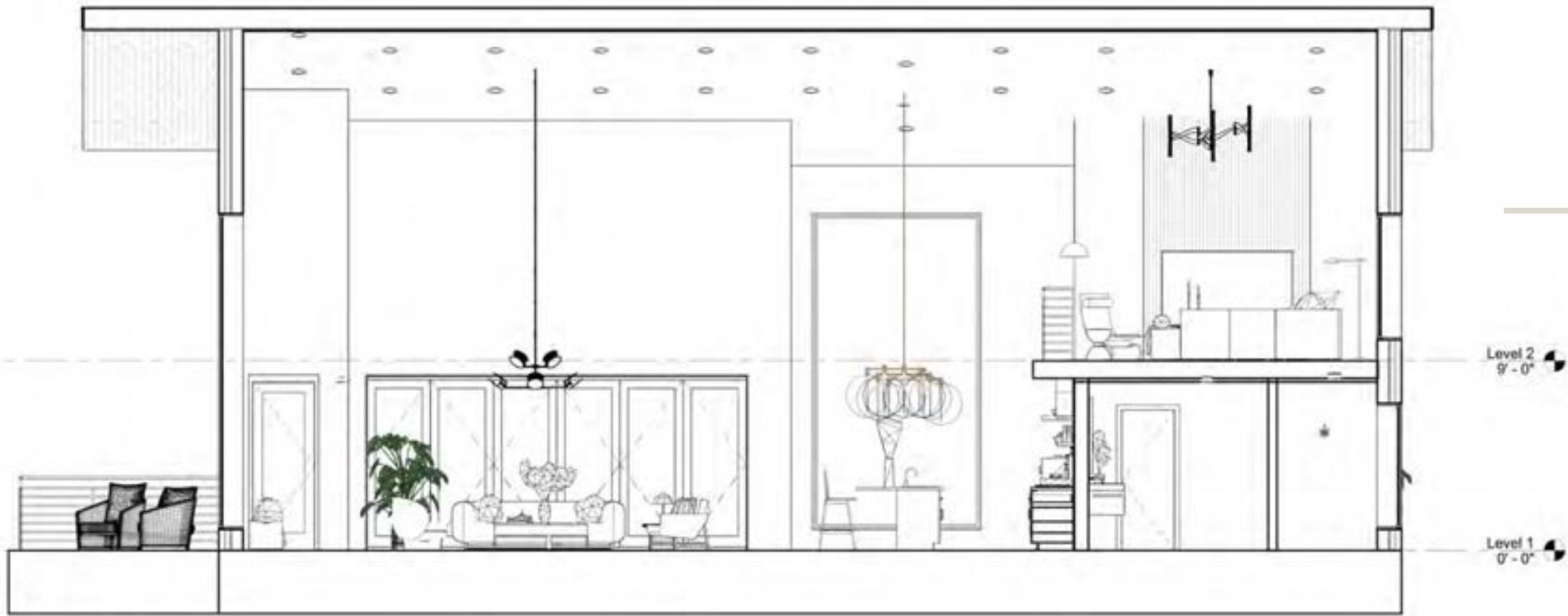
Wallace Nichols Guest House Section
