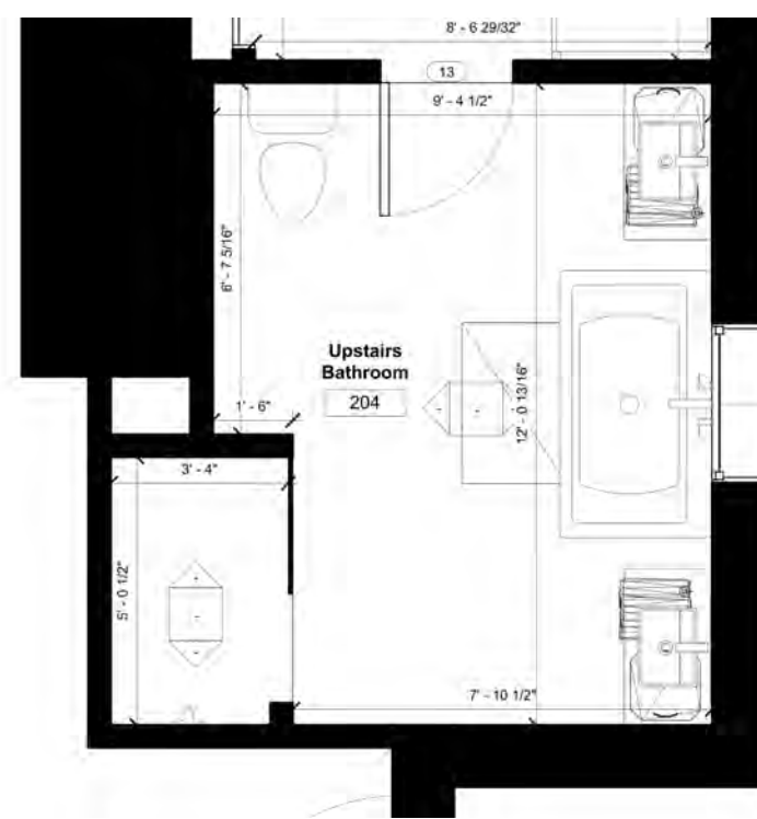
Upstairs Bathroom Floor Plan
