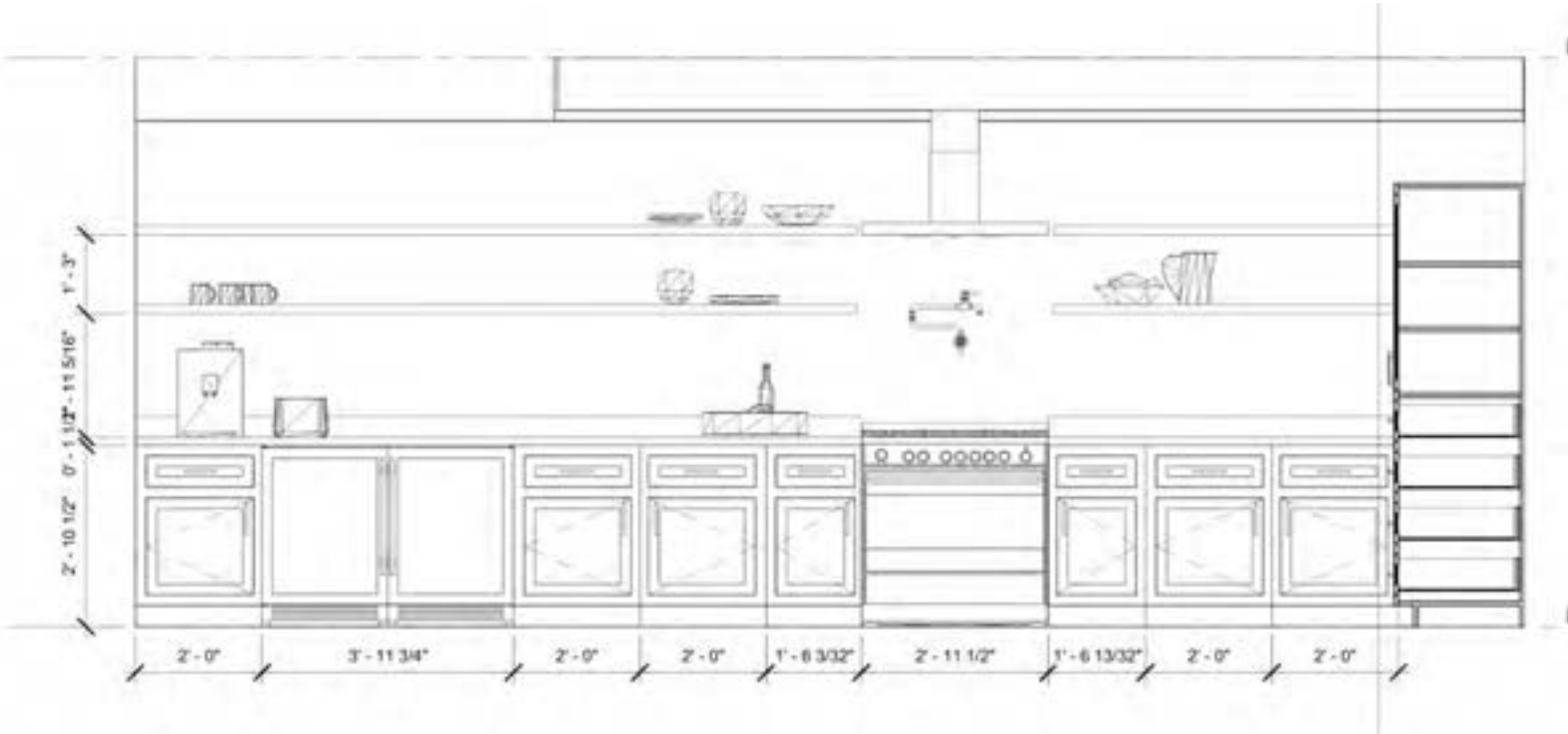
Kitchen Elevation - Long Side of Kitchen
