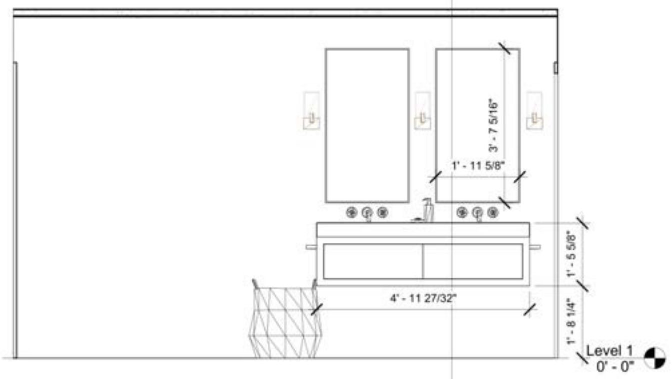
Primary Bathroom Elevation - Vanity
