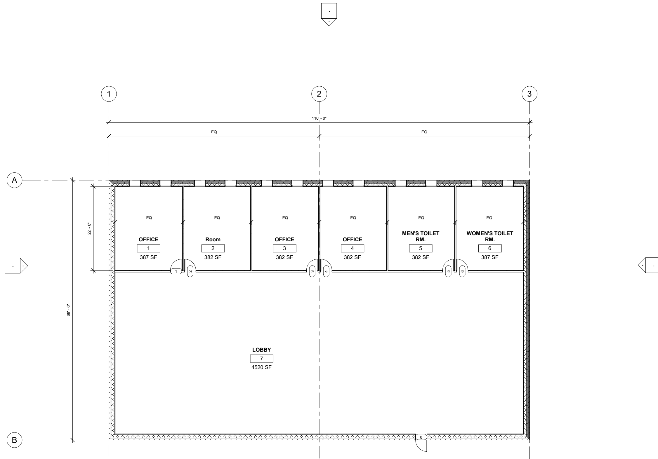
OFFICE BUILDING- Option A
