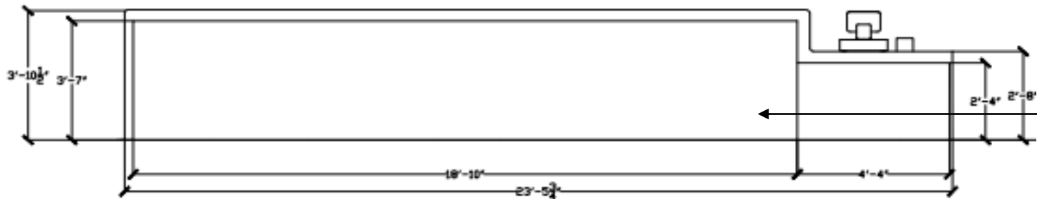
Bar Front View
