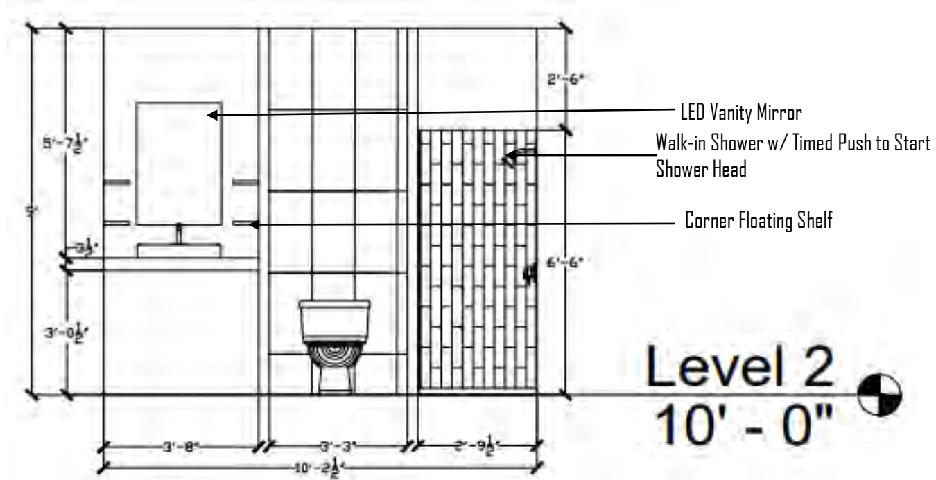
2nd Floor Bathroom Elevation
