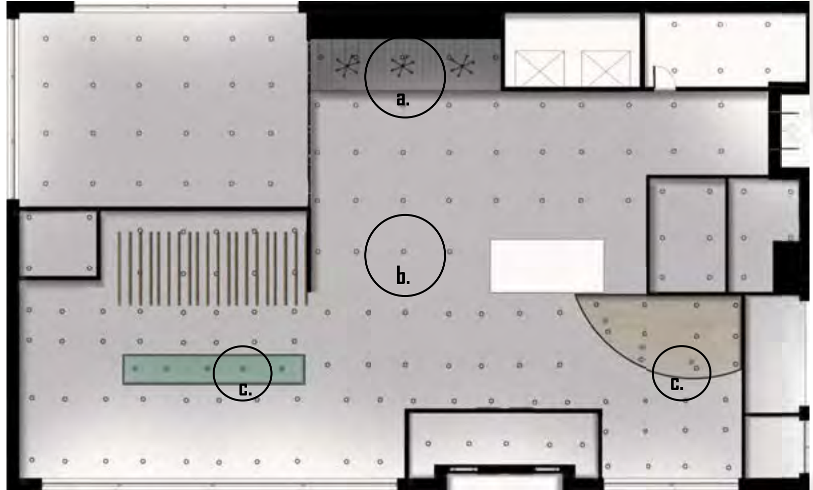
1st Floor Rendered Reflected Ceiling Plan
