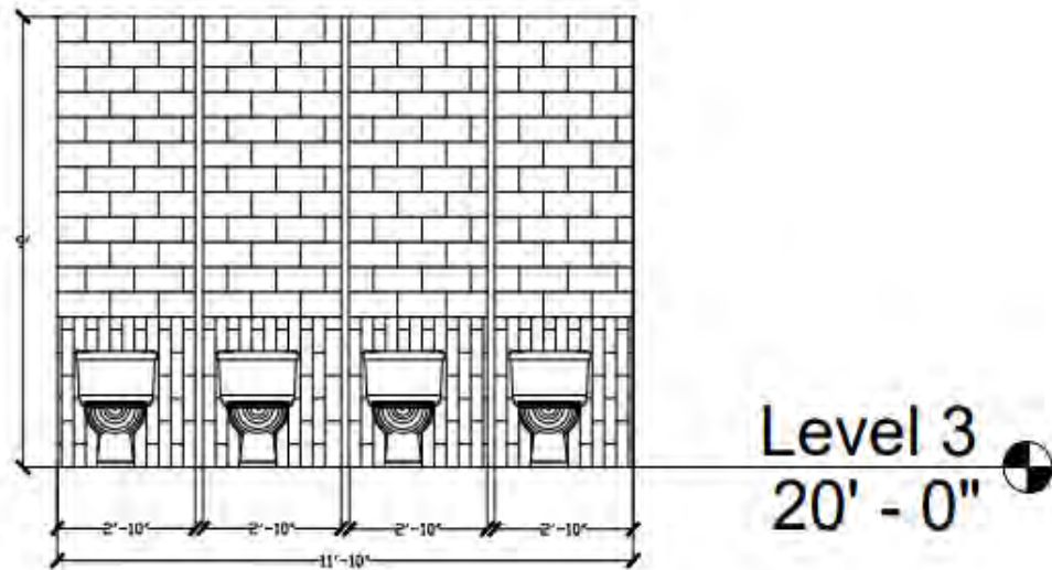
3rd Floor Stall Elevation
