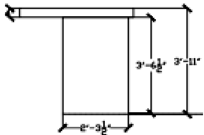
Bar Side View
