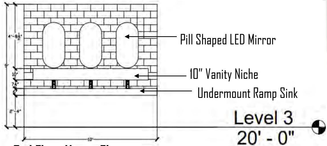
3rd Floor Vanity Elevation
