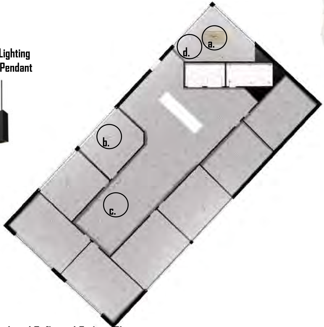
3rd Floor Rendered Reflected Ceiling Plan
