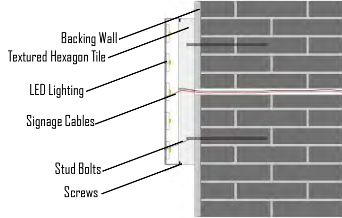
LED Backlit Sign Side View Diagram
